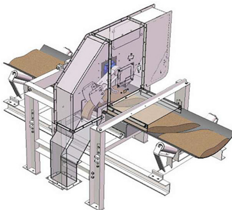
Figure 10.1: Cross Stream Sampler Schematic
