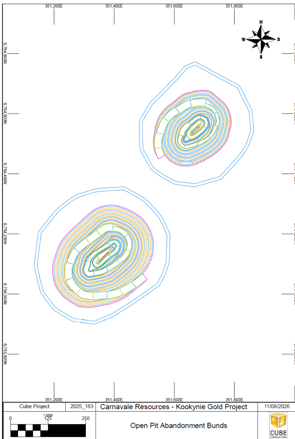
Figure 8.7: Abandonment bund design
