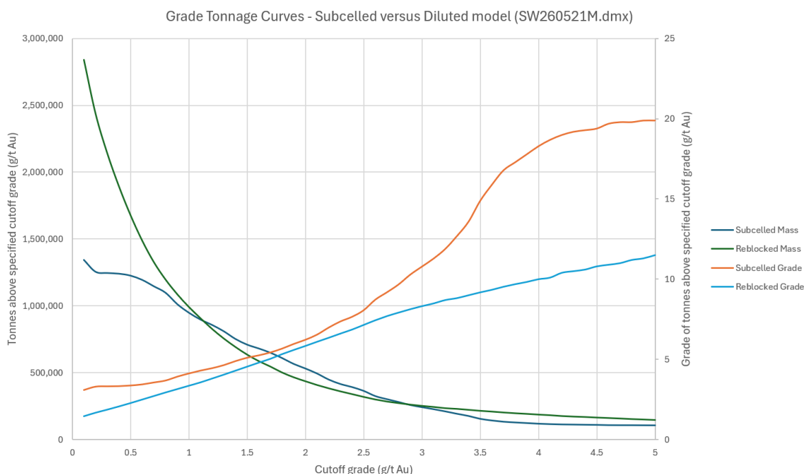
Figure 8.1: Grade-tonnage comparison of resource vs. diluted/regularised block model
