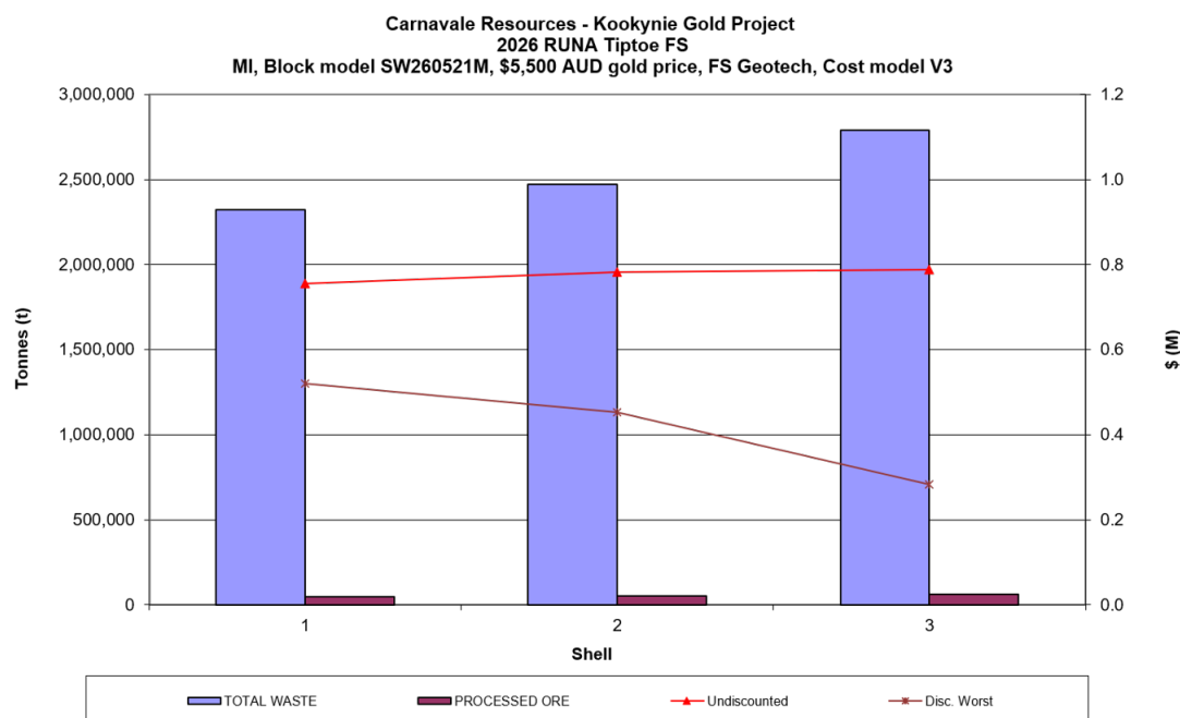
Figure 8.3: Tiptoe Run A tonnage / cashflow chart
