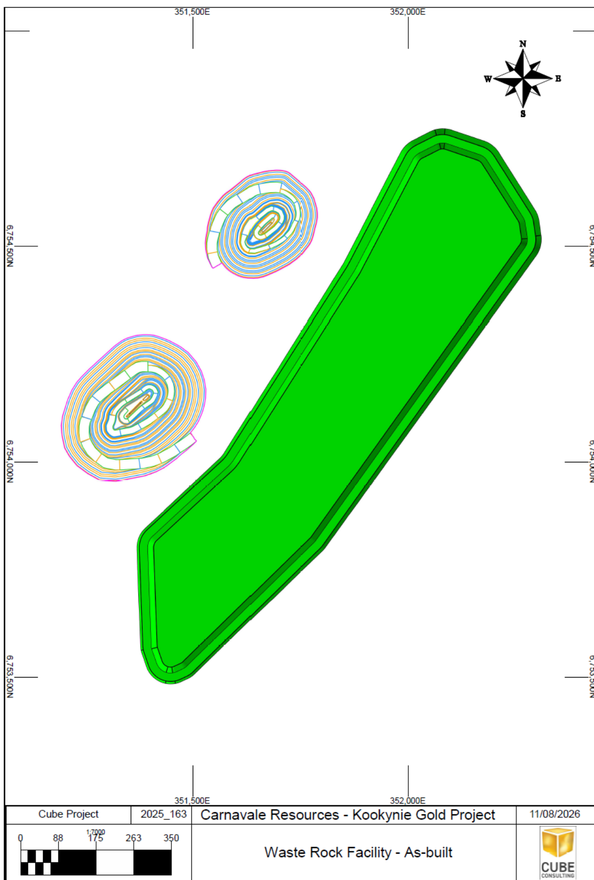
Figure 8.8: Kookynie Gold Project WRL as-built design, with final pit limits
