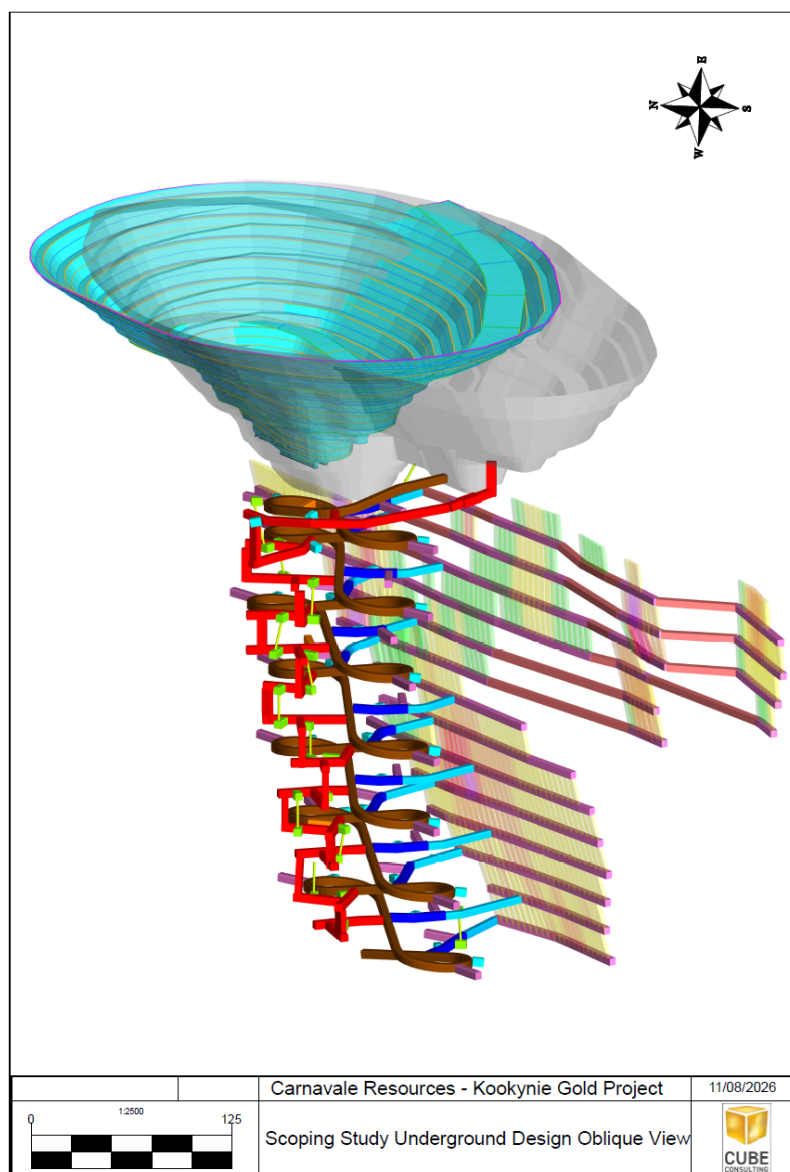
Figure11, Swiftsure BFS pit and Scoping Study Underground Design Oblique View Teal: Swiftsure Feasibility Study design. Grey: October 2025 Scoping Study design. Oblique view: Scoping Study underground design
