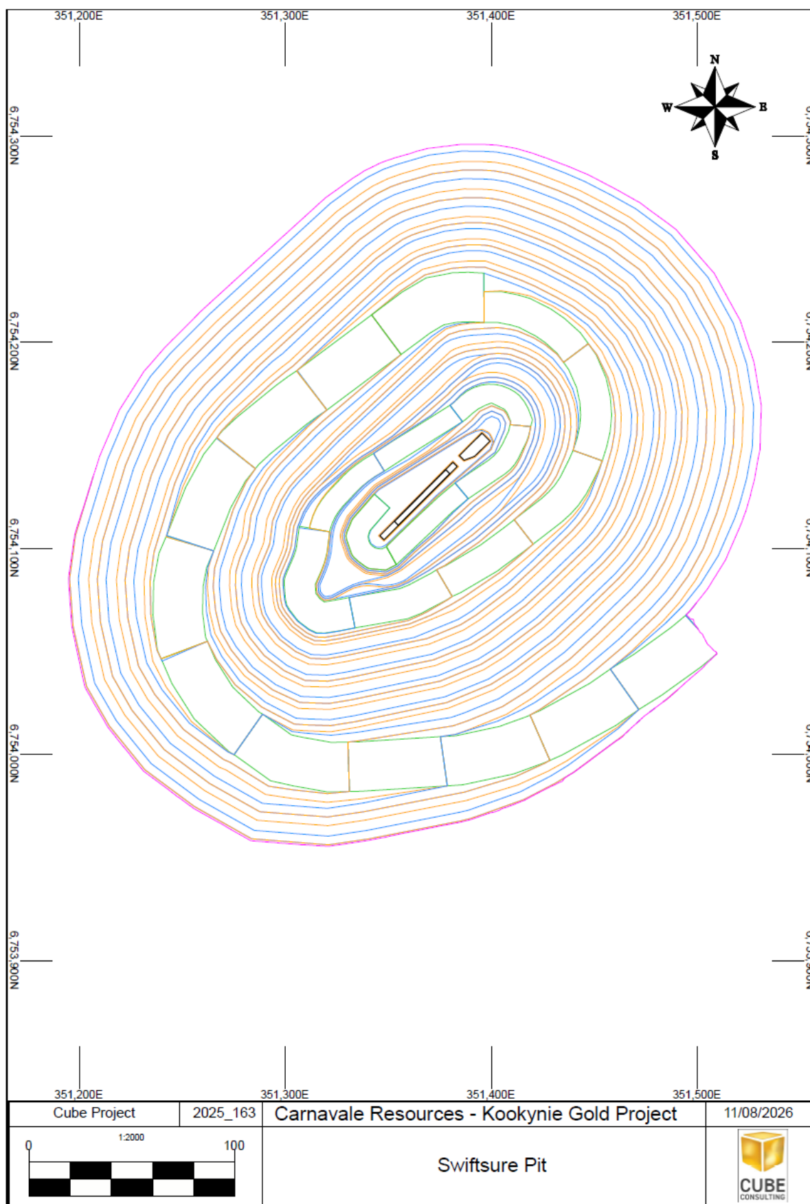
Figure 8.4: Swiftsure detailed pit design
