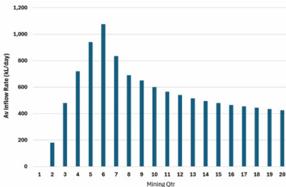
Figure 6.1: Base case results of inflows and water table drawdowns
