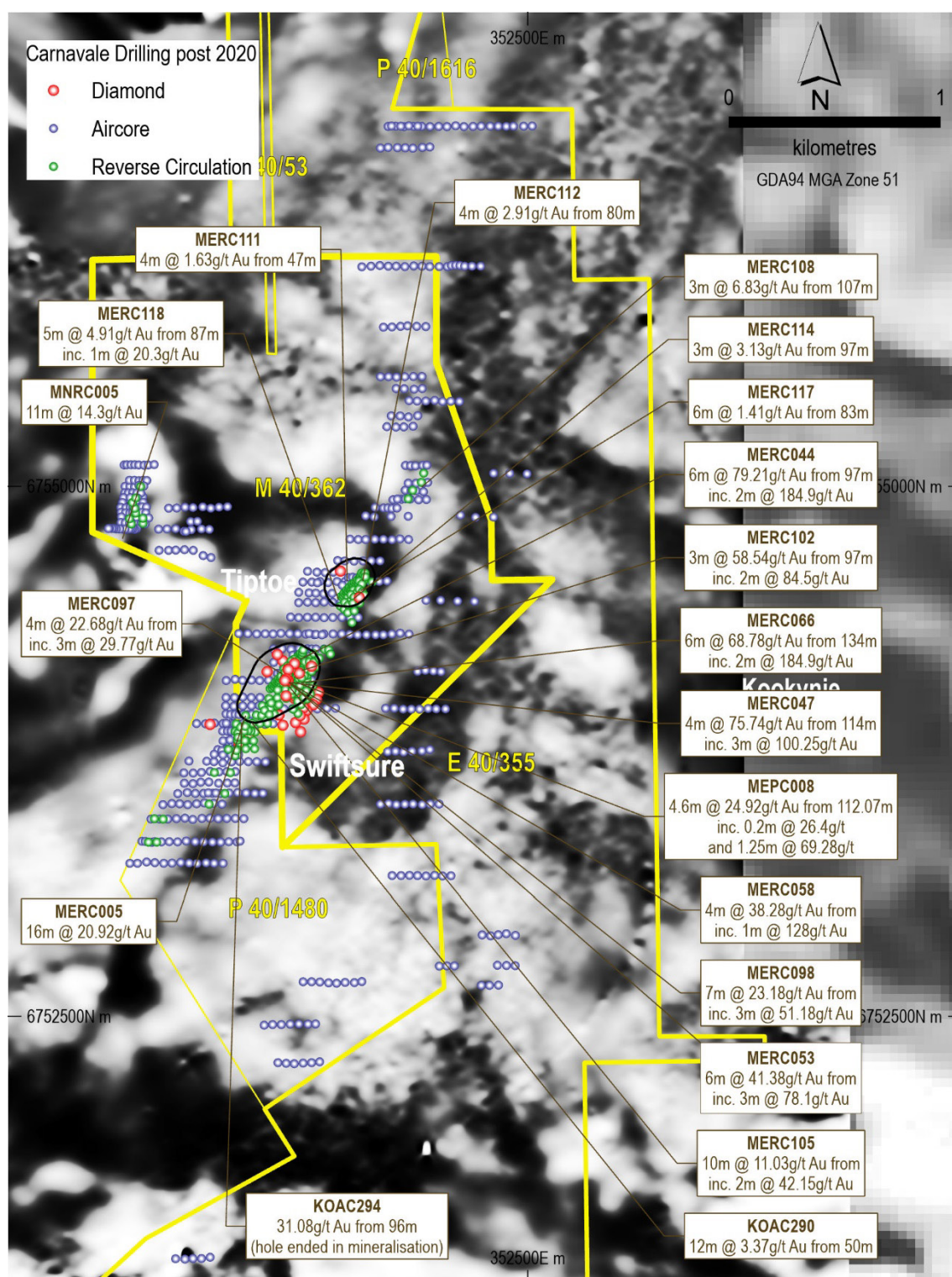
Figure 3.4: Drillhole location layout
