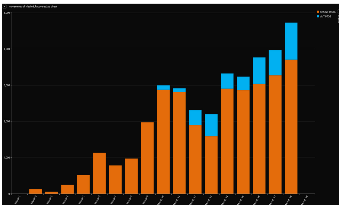
Figure 8.14: Recovered ounces by period – Run 4
