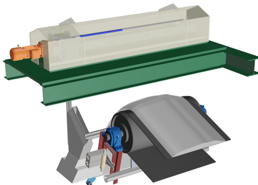
Figure 10.2: End of Stream Sampler Schematic
