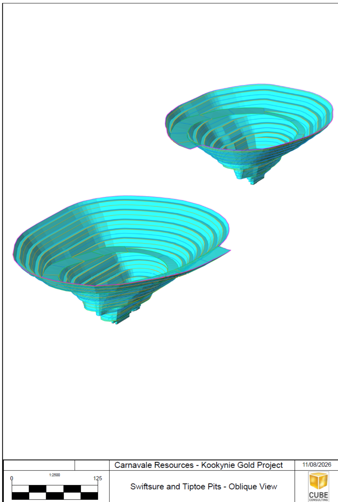
Figure 8.6: Swiftsure (bottom left) and Tiptoe (upper right) pits - oblique view
