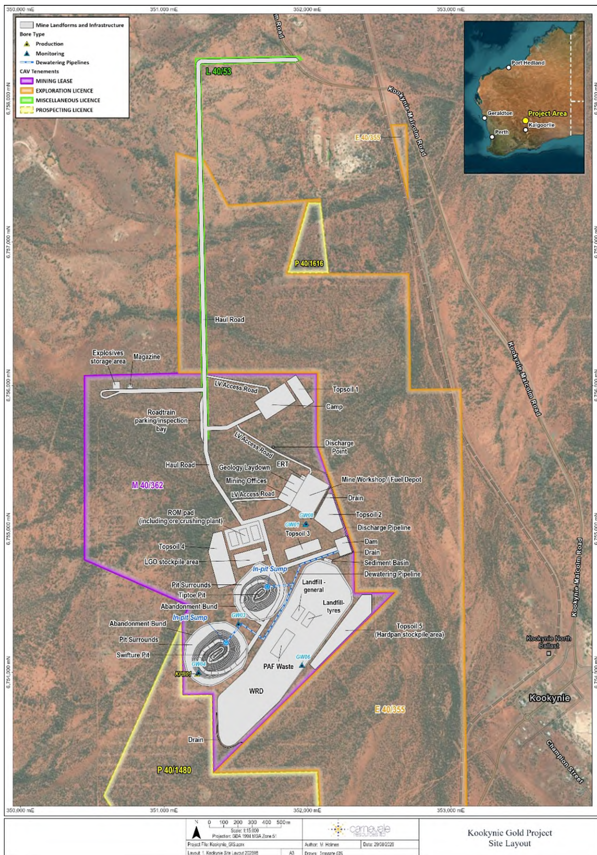
Figure 10, KGP BFS Site layout
