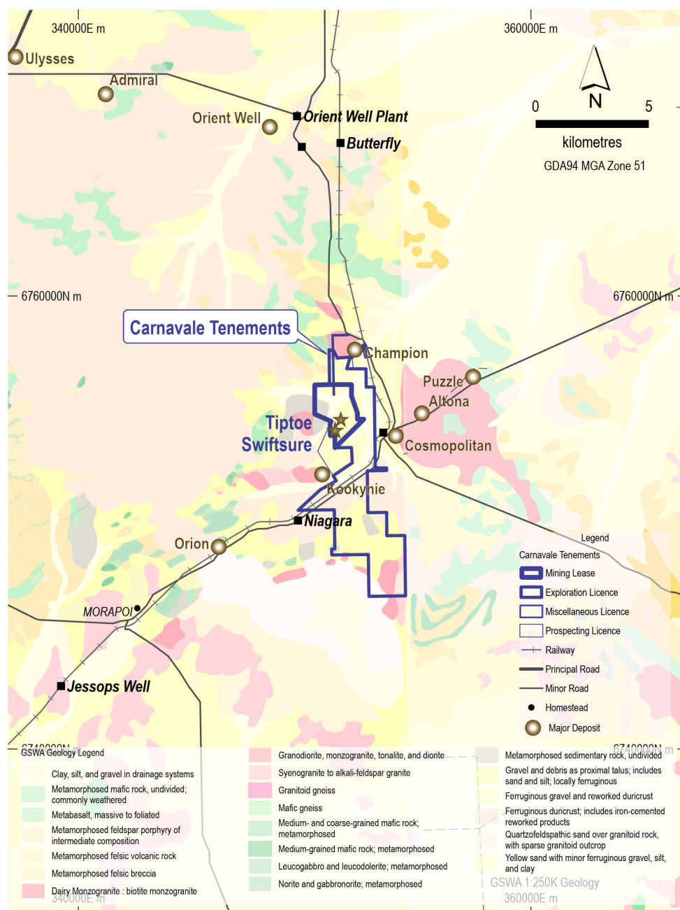
Figure 3.2: Regional Geology Map showing TT and SS
