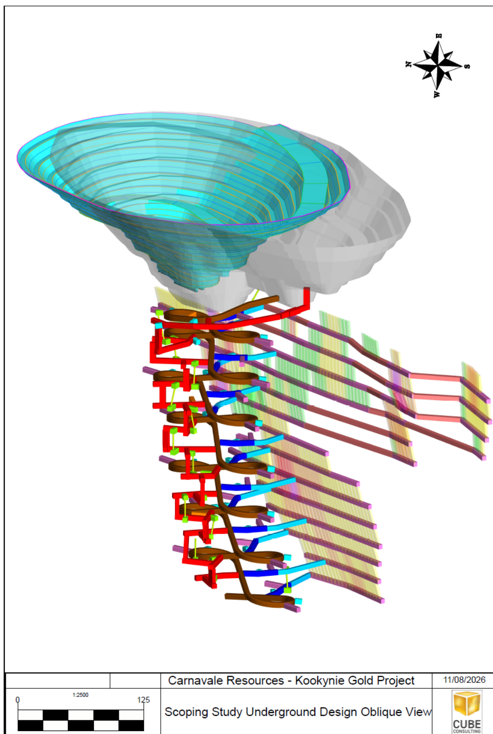
Figure 8.16: Scoping Study Underground Design Oblique View
