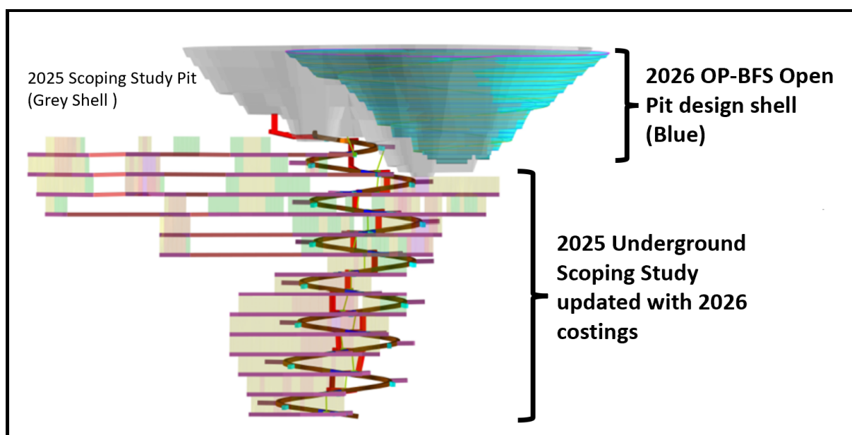
Figure 1 – Swiftsure Open Pit and Underground . BFS open pit design shell overlain on October 2025 Scoping Study pit shell and UG design
