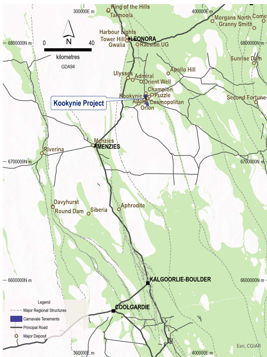
Figure 3.1: Regional Location Map showing Kookynie Project within Norseman-Wiluna Greenstone Belt
