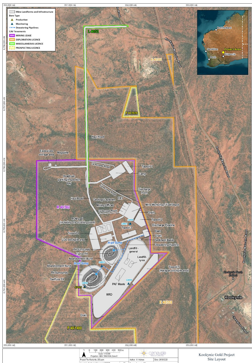
Figure 11.1: Project General Arrangement
