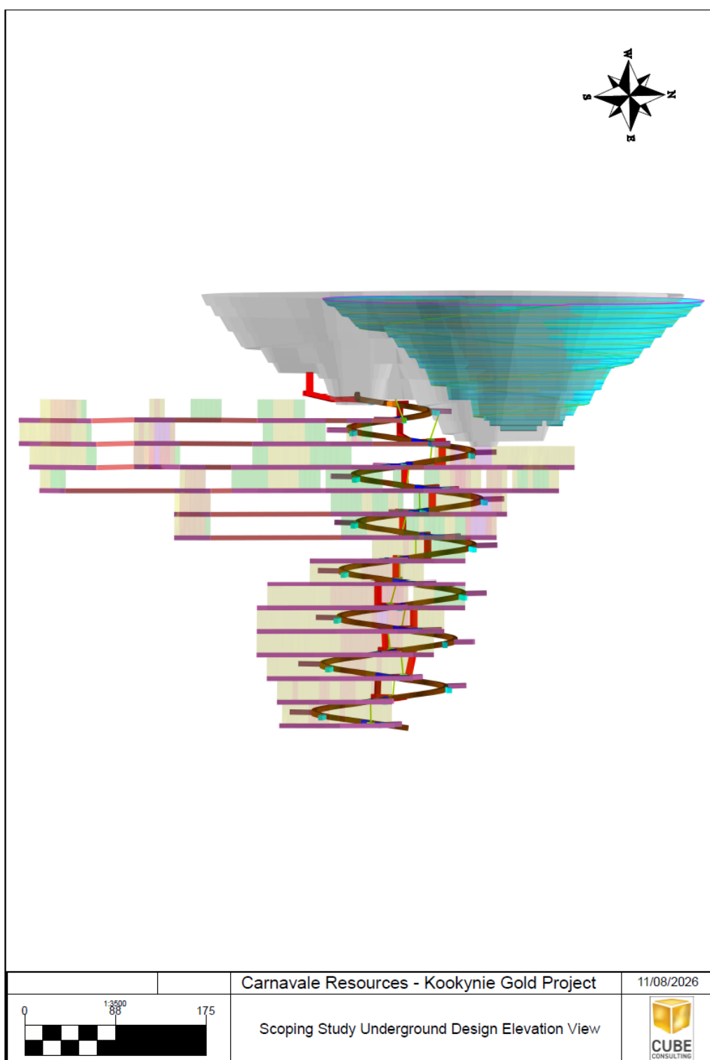
Figure 8.17: Scoping Study Underground Design Elevation View
