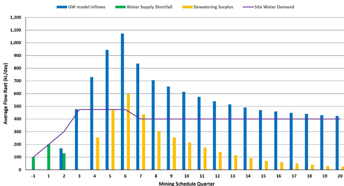
Figure 6.2: Project water balance
