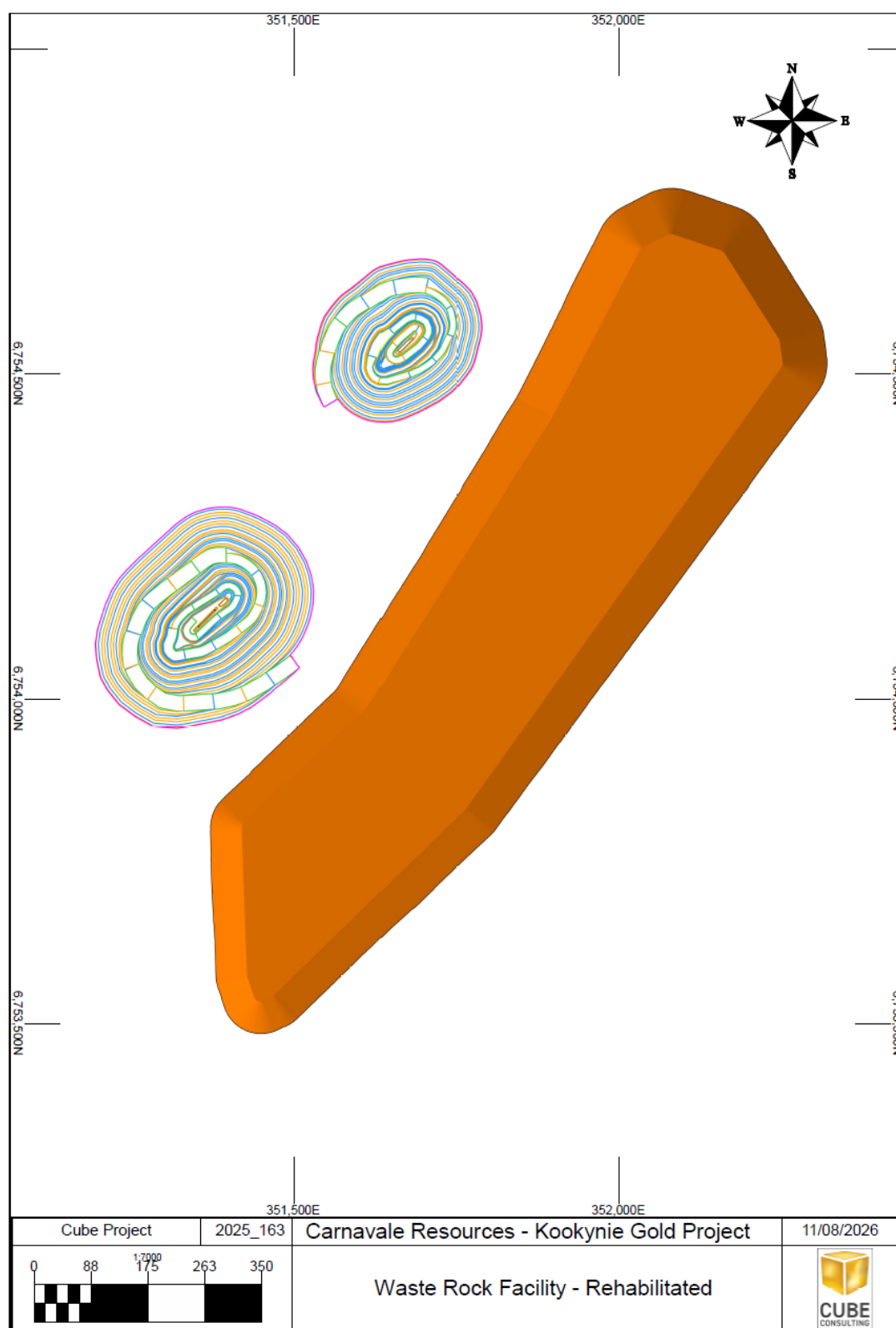
Figure 8.9: Kookynie Gold Project WRL rehabilitated design, with final pit limits
