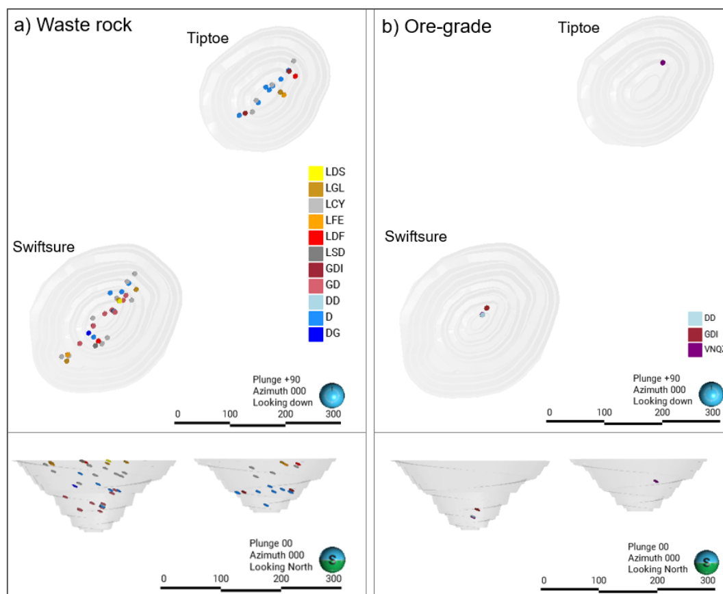
Figure 5.1: Sample locations
