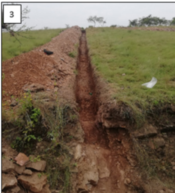
Figure 4 Photos 3 & 4 - Cassiterite in trench from Hippo Hill (Cassiterite visually estimated to be <1% in samples by volume)
